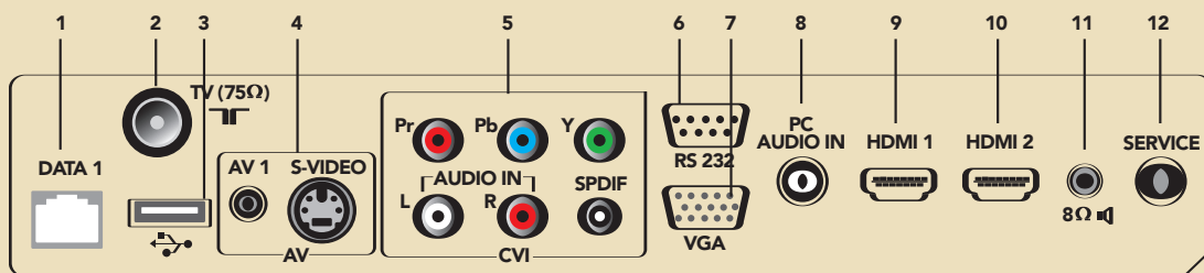
REAR JACK PANEL 1. Smart Port Jack; 2. TV Aerial; 3. USB; 4. AV Input (Composite & S-Video); 5. CVI (Component Video Input); 6. Control Jack; 7. VGA Input; 8. PC Audio Input; 9. HDMI; 10. HDMI; 11. Pillow Speaker Input
